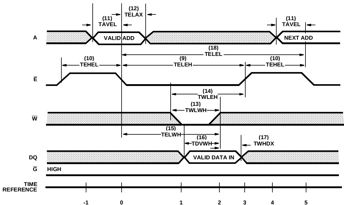
FIGURE 2. WRITE CYCLE
