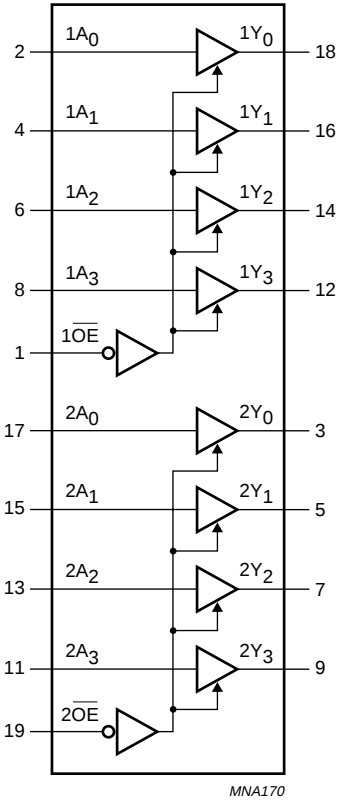
Fig.3 Logic diagram.
