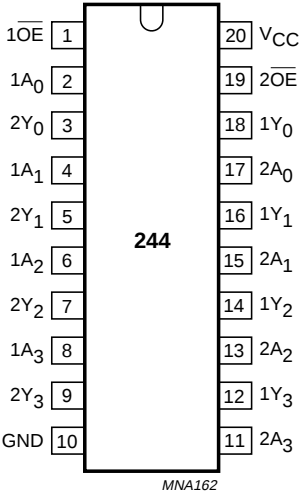
Fig.1 Pin configuration.
